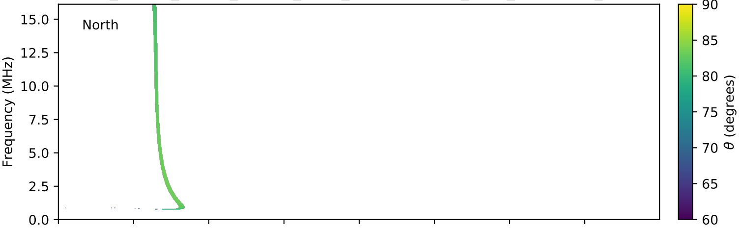
expres_cassini_jupiter_europa_isaac_lossc-wid1deg_3kev_20010515_v01.cdf
