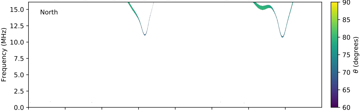
expres_cassini_jupiter_europa_isaac_lossc-wid1deg_3kev_20010514_v01.cdf
