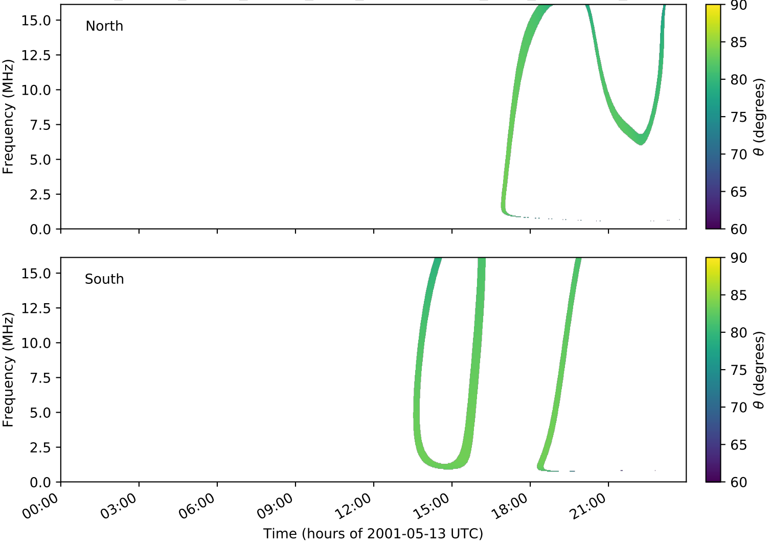
expres_cassini_jupiter_europa_isaac_lossc-wid1deg_3kev_20010513_v01.cdf
