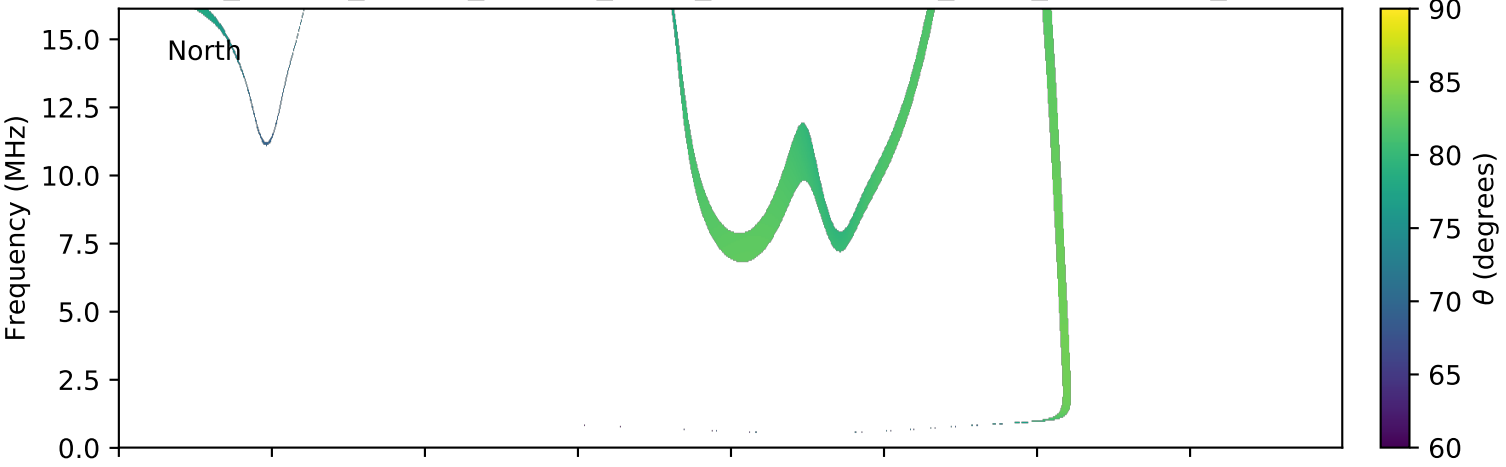
expres_cassini_jupiter_europa_isaac_lossc-wid1deg_3kev_20010511_v01.cdf
