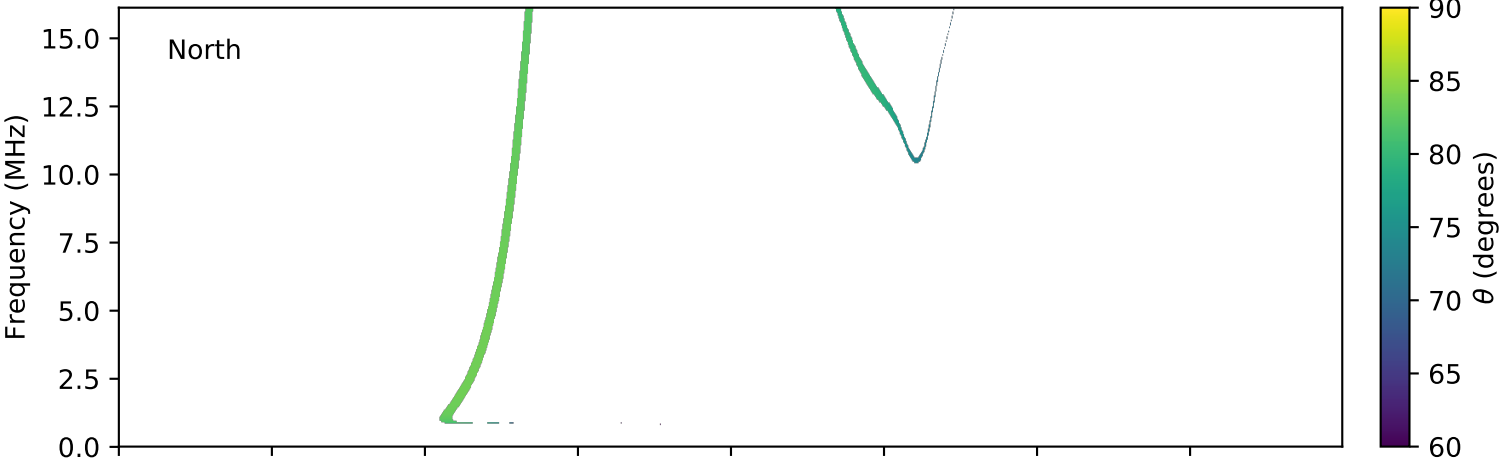
expres_cassini_jupiter_europa_isaac_lossc-wid1deg_3kev_20010510_v01.cdf
