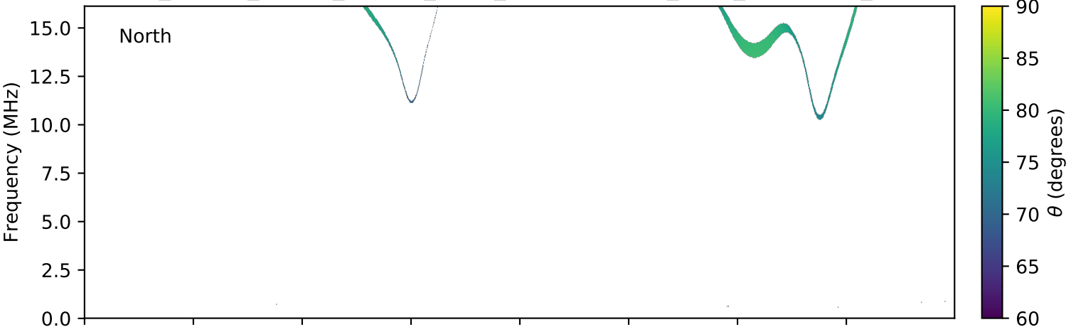
expres_cassini_jupiter_europa_isaac_lossc-wid1deg_3kev_20010507_v01.cdf
