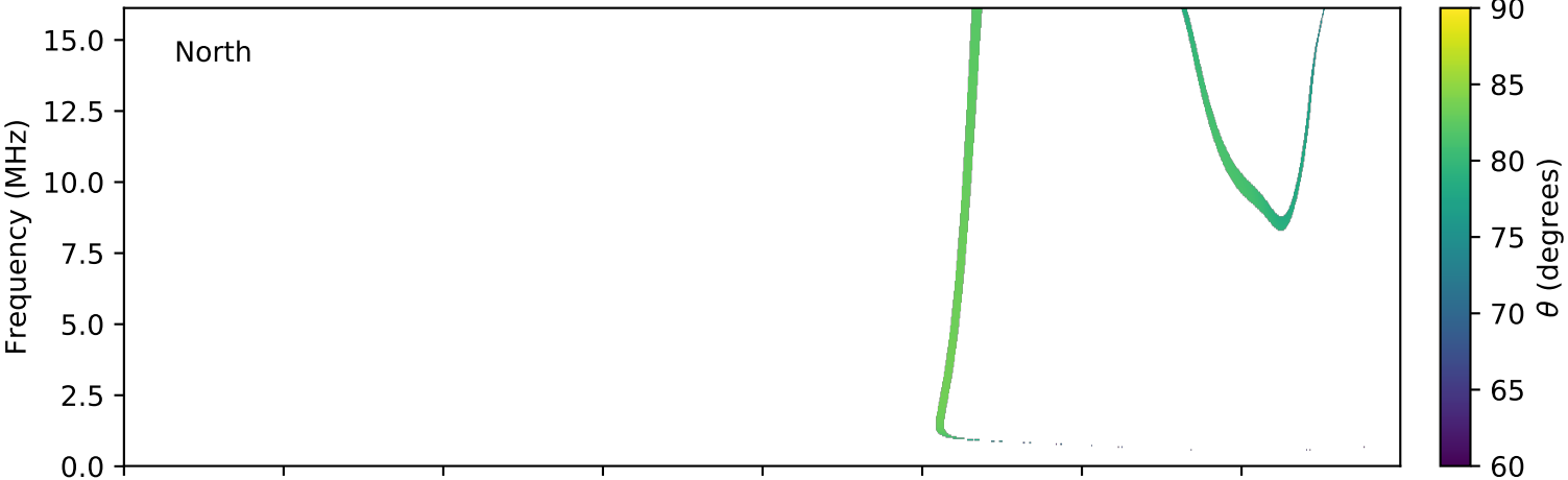
expres_cassini_jupiter_europa_isaac_lossc-wid1deg_3kev_20010506_v01.cdf
