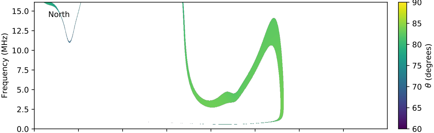
expres_cassini_jupiter_europa_isaac_lossc-wid1deg_3kev_20010504_v01.cdf
