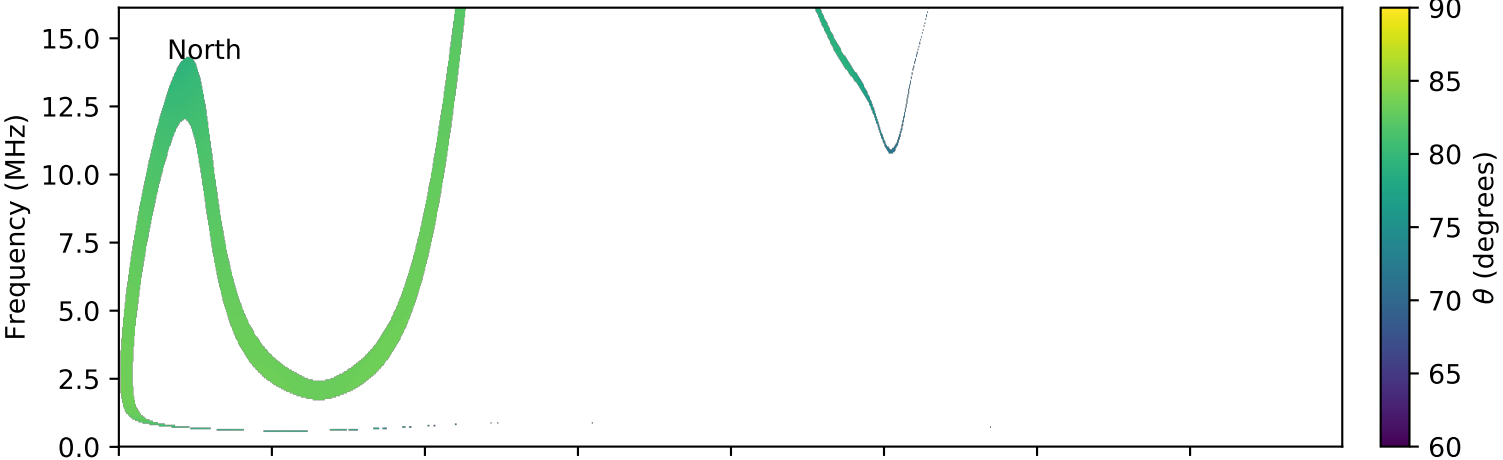
expres_cassini_jupiter_europa_isaac_lossc-wid1deg_3kev_20010503_v01.cdf
