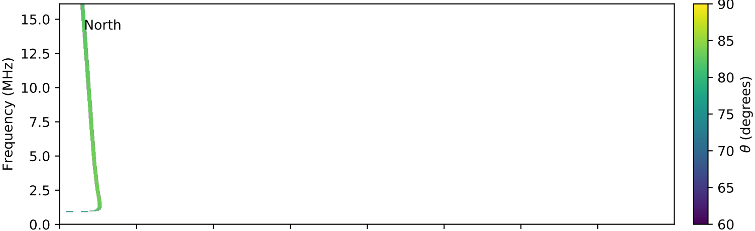
expres_cassini_jupiter_europa_isaac_lossc-wid1deg_3kev_20010501_v01.cdf
