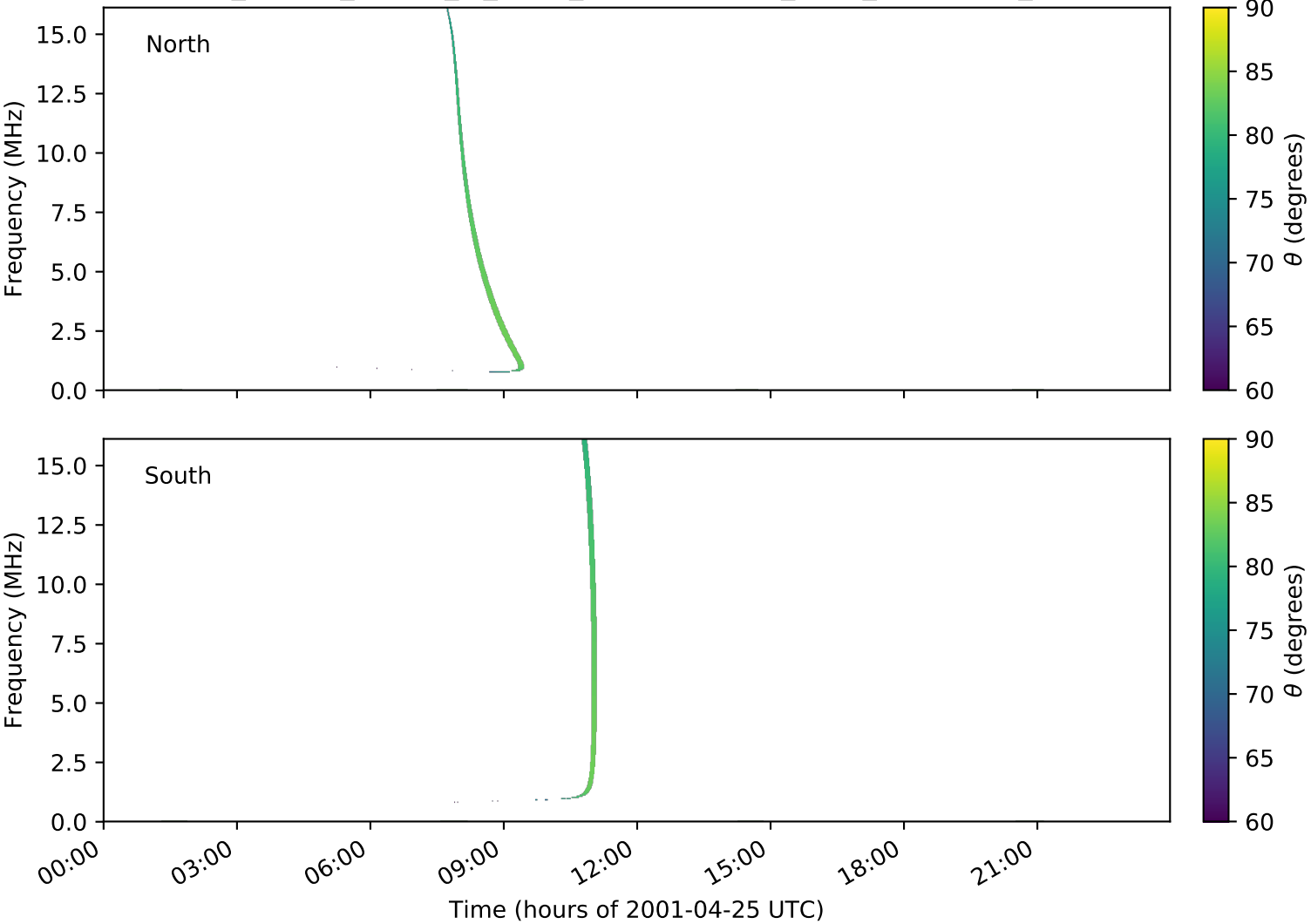
expres_cassini_jupiter_io_isaac_lossc-wid1deg_3kev_20010425_v01.cdf
