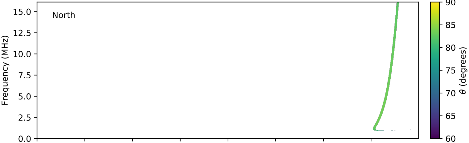
expres_cassini_jupiter_io_isaac_lossc-wid1deg_3kev_20010422_v01.cdf
