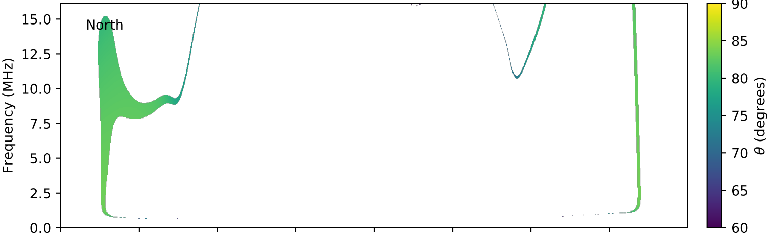
expres_cassini_jupiter_io_isaac_lossc-wid1deg_3kev_20010421_v01.cdf
