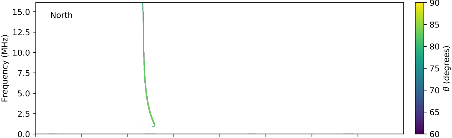
expres_cassini_jupiter_io_isaac_lossc-wid1deg_3kev_20010418_v01.cdf
