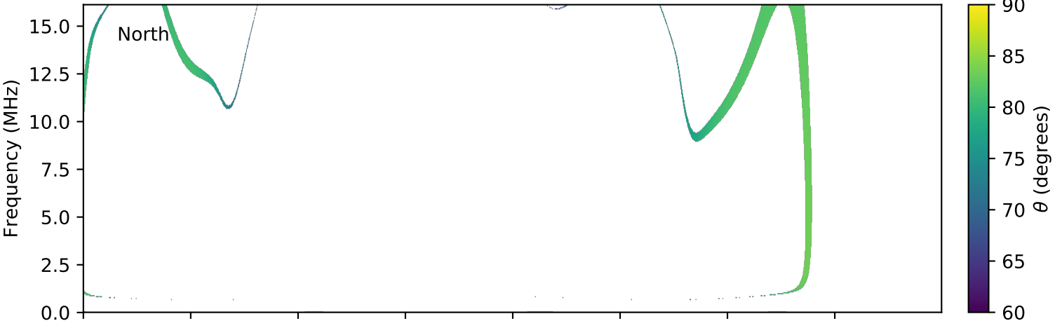
expres_cassini_jupiter_io_isaac_lossc-wid1deg_3kev_20010414_v01.cdf
