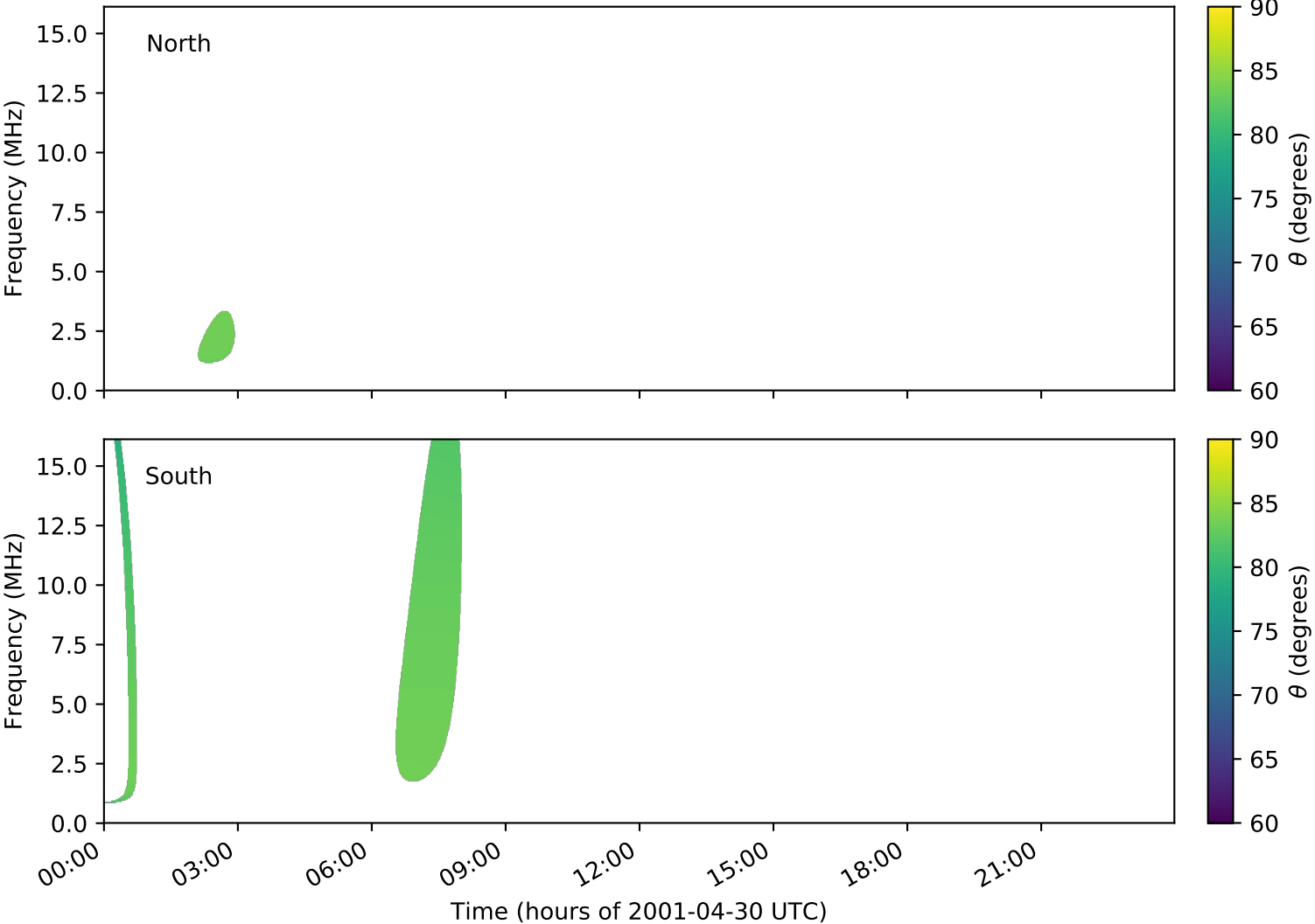
expres_cassini_jupiter_ganymede_isaac_lossc-wid1deg_3kev_20010430_v01.cdf
