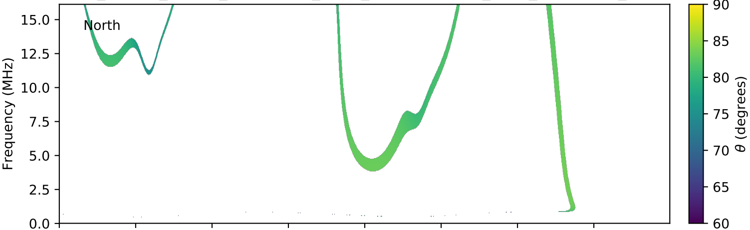
expres_cassini_jupiter_ganymede_isaac_lossc-wid1deg_3kev_20010429_v01.cdf
