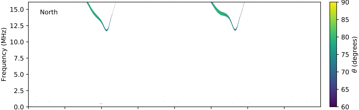
expres_cassini_jupiter_ganymede_isaac_lossc-wid1deg_3kev_20010428_v01.cdf
