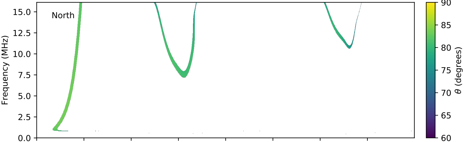
expres_cassini_jupiter_ganymede_isaac_lossc-wid1deg_3kev_20010427_v01.cdf
