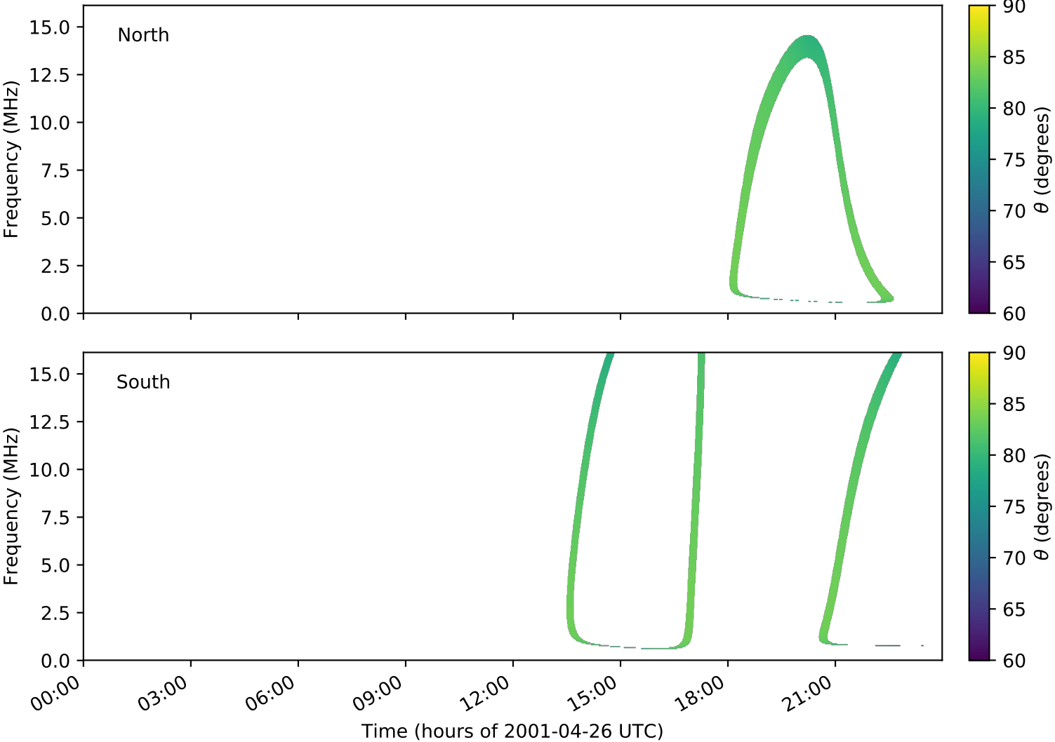
expres_cassini_jupiter_ganymede_isaac_lossc-wid1deg_3kev_20010426_v01.cdf
