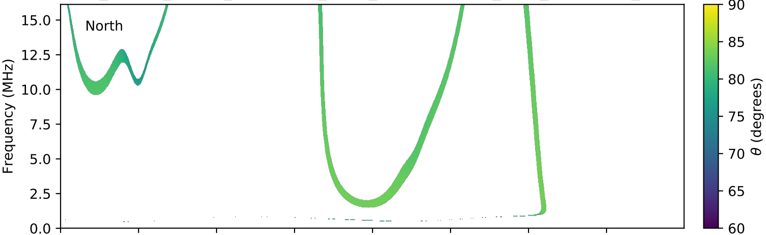
expres_cassini_jupiter_ganymede_isaac_lossc-wid1deg_3kev_20010422_v01.cdf
