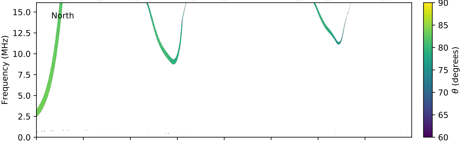
expres_cassini_jupiter_ganymede_isaac_lossc-wid1deg_3kev_20010420_v01.cdf
