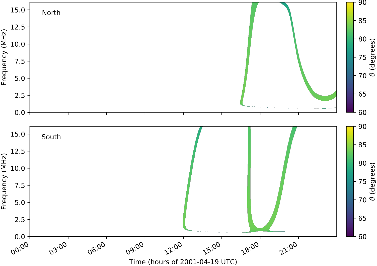
expres_cassini_jupiter_ganymede_isaac_lossc-wid1deg_3kev_20010419_v01.cdf
