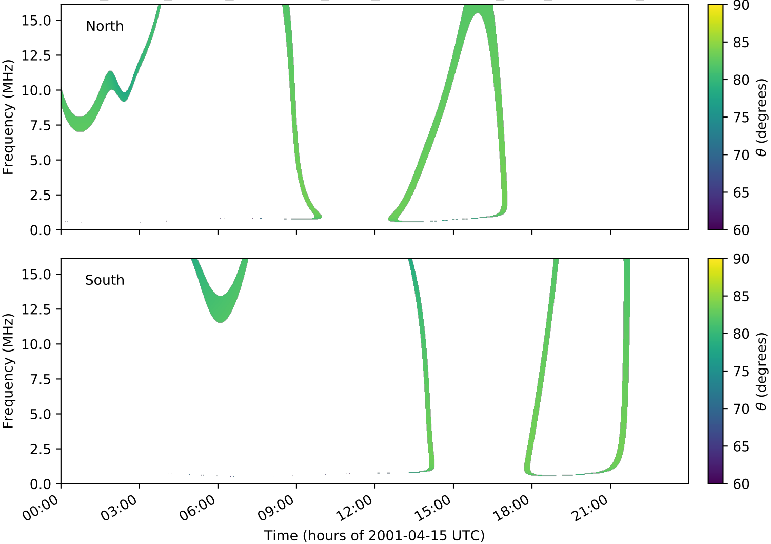
expres_cassini_jupiter_ganymede_isaac_lossc-wid1deg_3kev_20010415_v01.cdf
