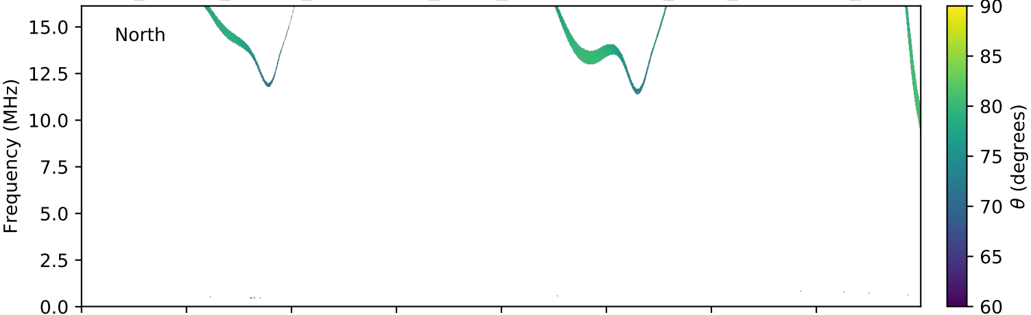
expres_cassini_jupiter_ganymede_isaac_lossc-wid1deg_3kev_20010414_v01.cdf
