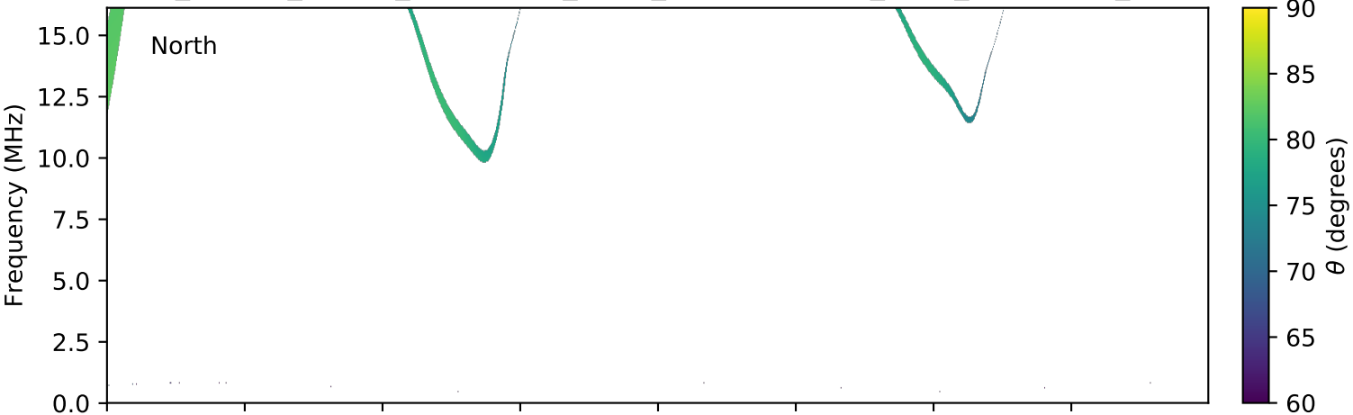
expres_cassini_jupiter_ganymede_isaac_lossc-wid1deg_3kev_20010413_v01.cdf
