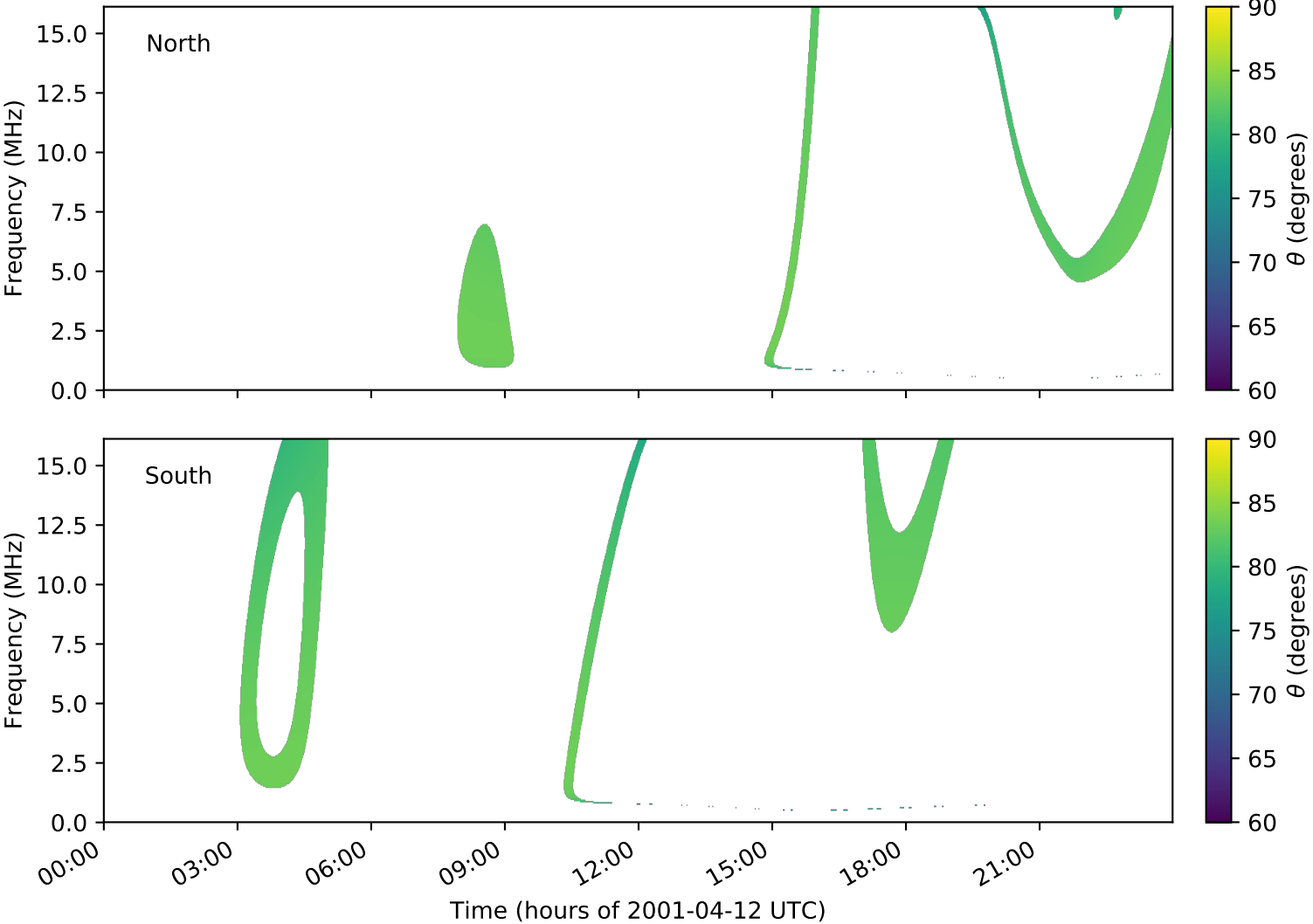
expres_cassini_jupiter_ganymede_isaac_lossc-wid1deg_3kev_20010412_v01.cdf
