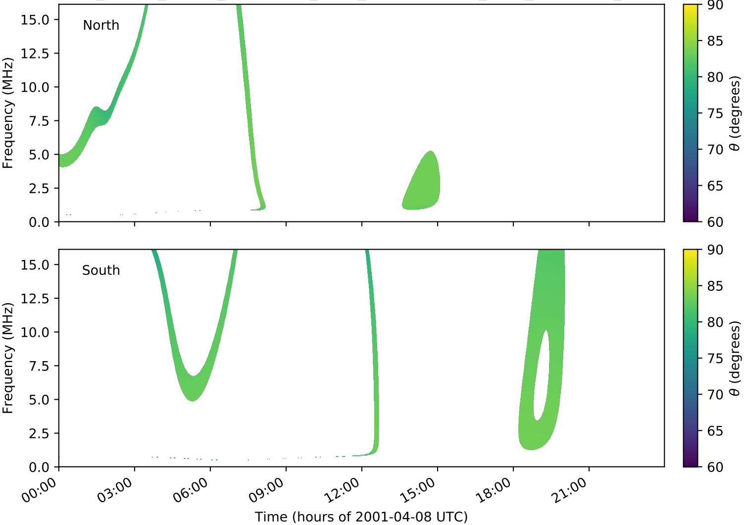
expres_cassini_jupiter_ganymede_isaac_lossc-wid1deg_3kev_20010408_v01.cdf
