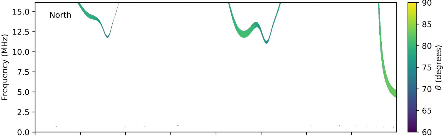
expres_cassini_jupiter_ganymede_isaac_lossc-wid1deg_3kev_20010407_v01.cdf
