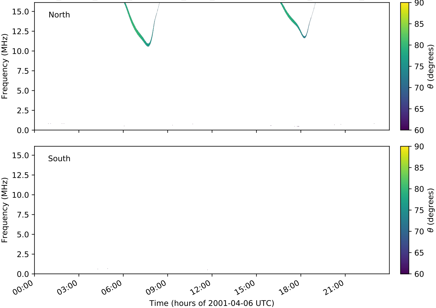
expres_cassini_jupiter_ganymede_isaac_lossc-wid1deg_3kev_20010406_v01.cdf
