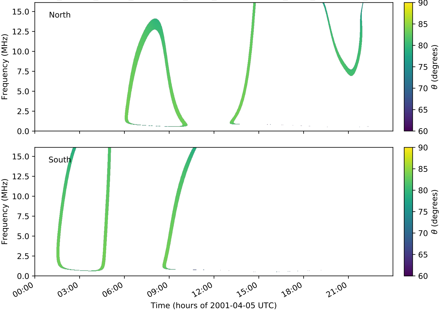
expres_cassini_jupiter_ganymede_isaac_lossc-wid1deg_3kev_20010405_v01.cdf
