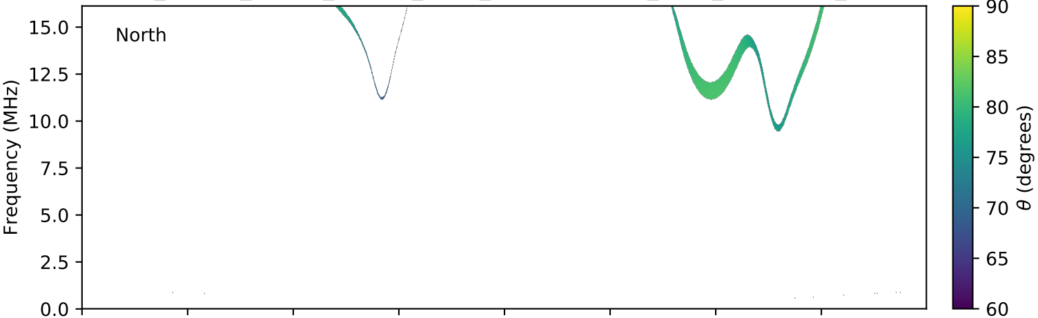
expres_cassini_jupiter_europa_isaac_lossc-wid1deg_3kev_20010430_v01.cdf
