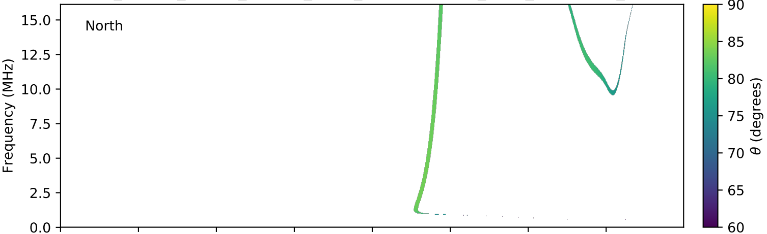
expres_cassini_jupiter_europa_isaac_lossc-wid1deg_3kev_20010429_v01.cdf
