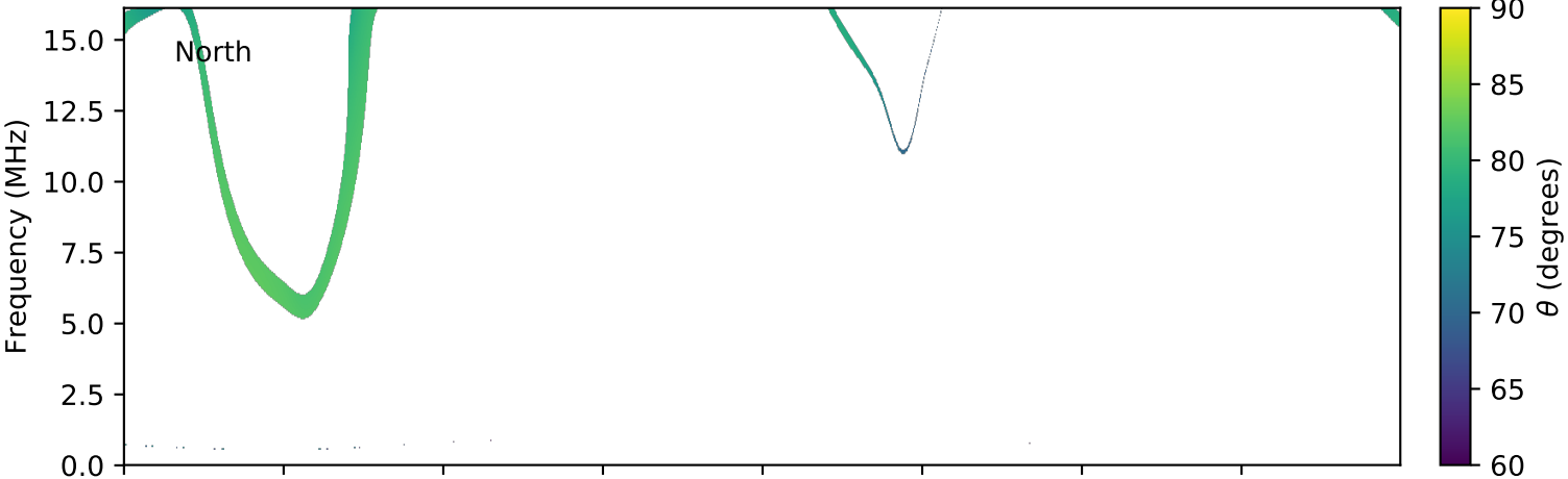
expres_cassini_jupiter_europa_isaac_lossc-wid1deg_3kev_20010426_v01.cdf
