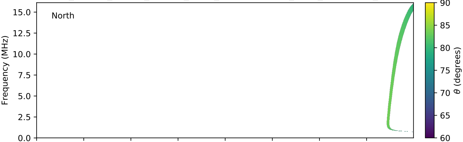
expres_cassini_jupiter_europa_isaac_lossc-wid1deg_3kev_20010425_v01.cdf
