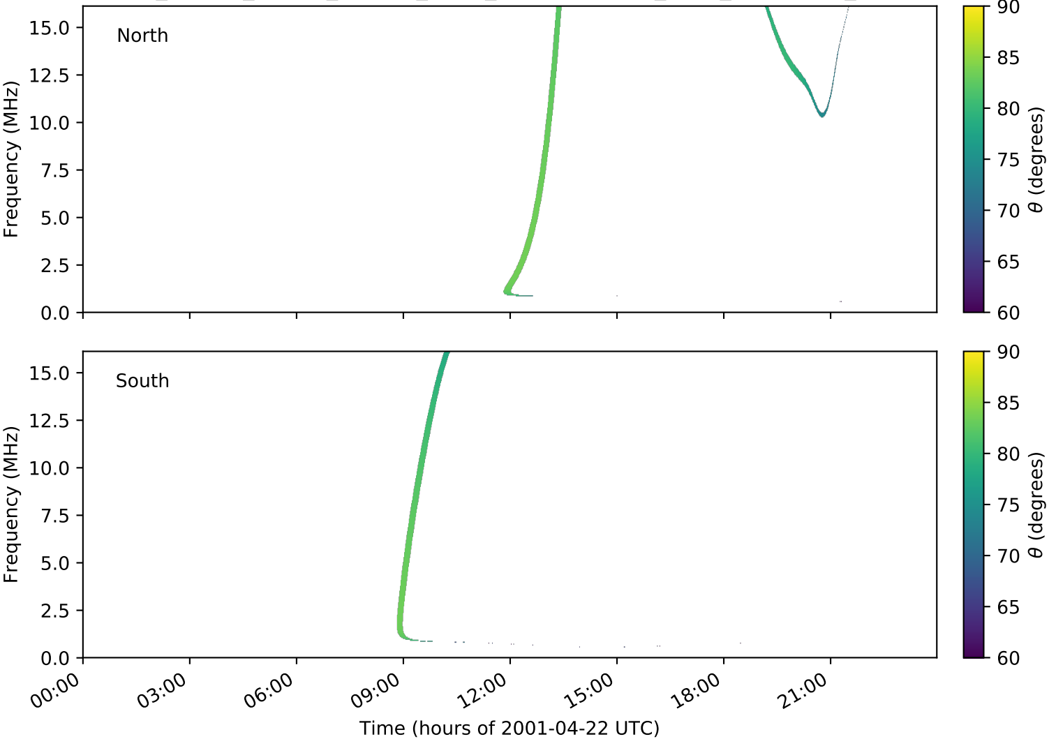
expres_cassini_jupiter_europa_isaac_lossc-wid1deg_3kev_20010422_v01.cdf
