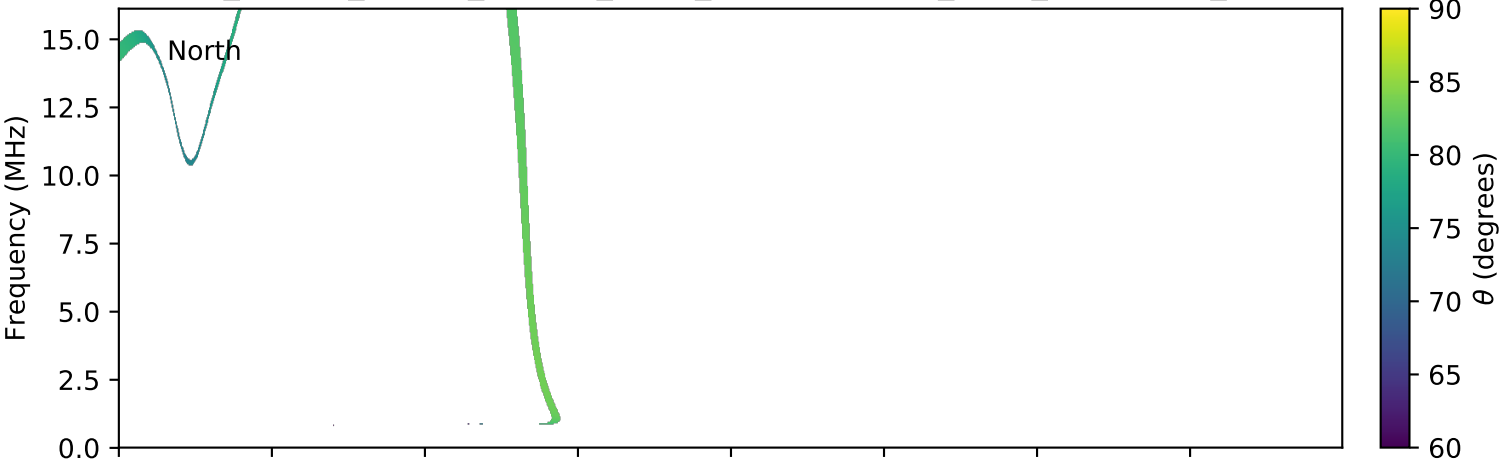
expres_cassini_jupiter_europa_isaac_lossc-wid1deg_3kev_20010420_v01.cdf
