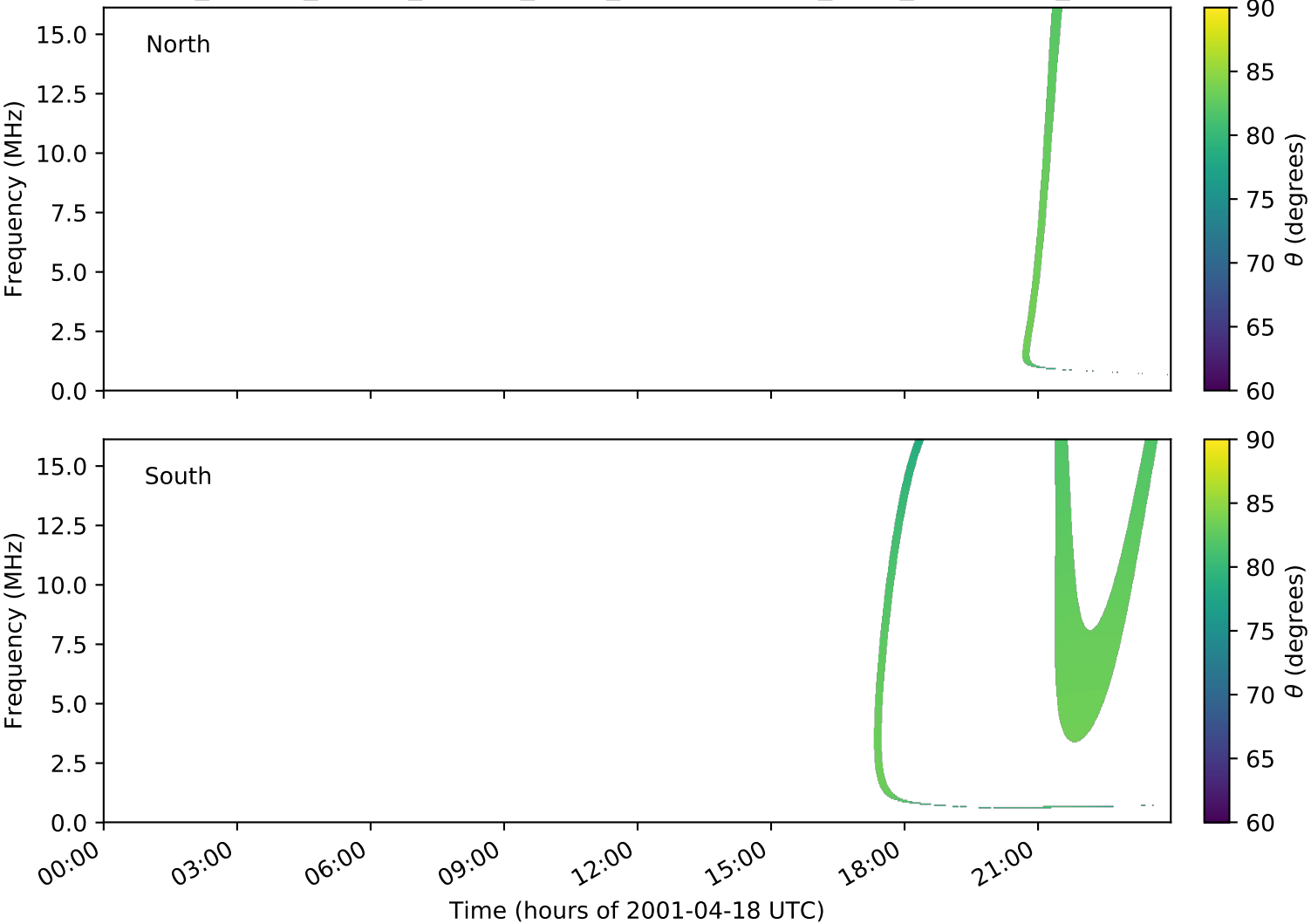
expres_cassini_jupiter_europa_isaac_lossc-wid1deg_3kev_20010418_v01.cdf
