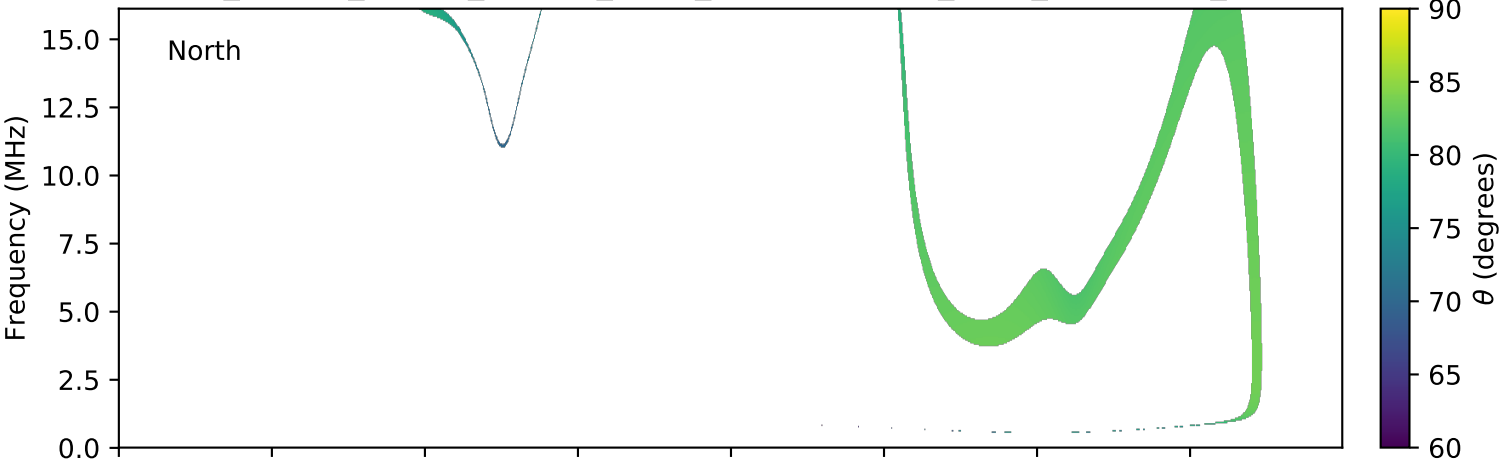
expres_cassini_jupiter_europa_isaac_lossc-wid1deg_3kev_20010416_v01.cdf
