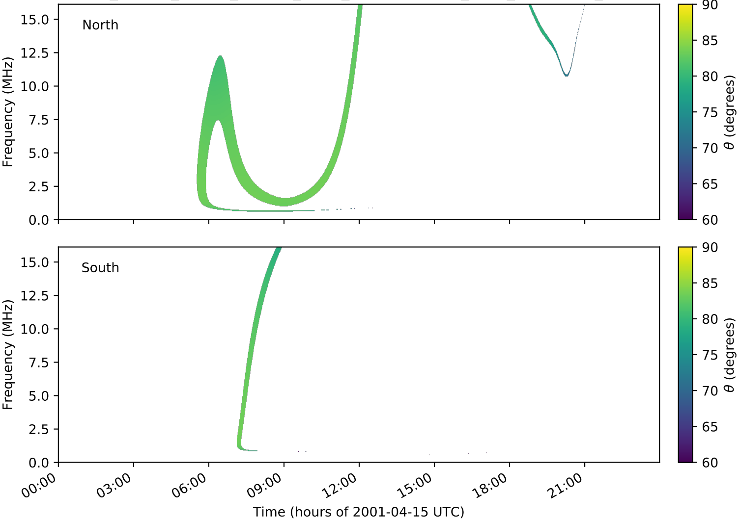
expres_cassini_jupiter_europa_isaac_lossc-wid1deg_3kev_20010415_v01.cdf
