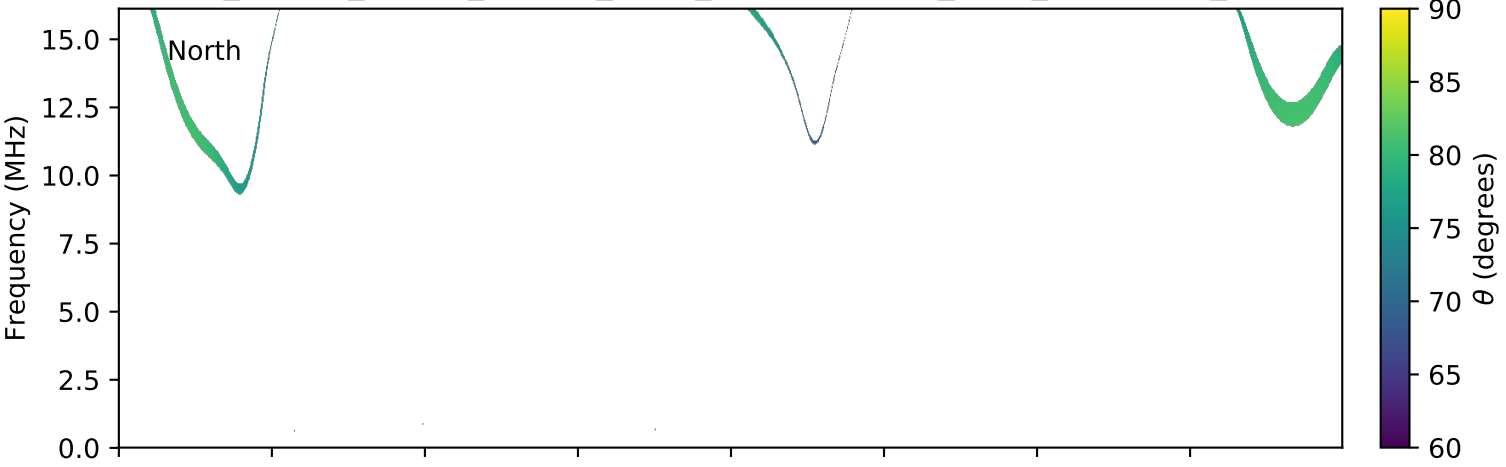
expres_cassini_jupiter_europa_isaac_lossc-wid1deg_3kev_20010412_v01.cdf
