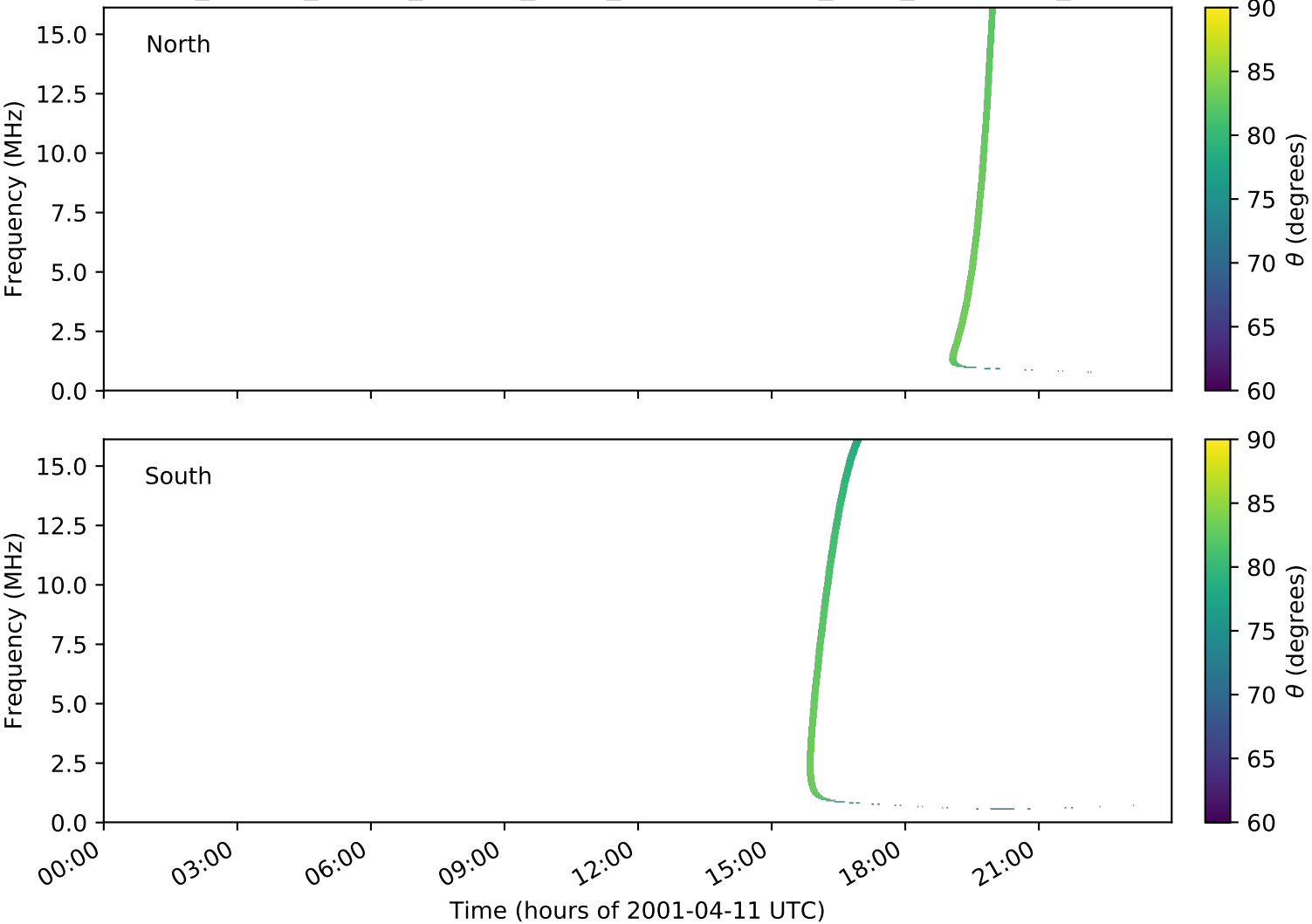
expres_cassini_jupiter_europa_isaac_lossc-wid1deg_3kev_20010411_v01.cdf
