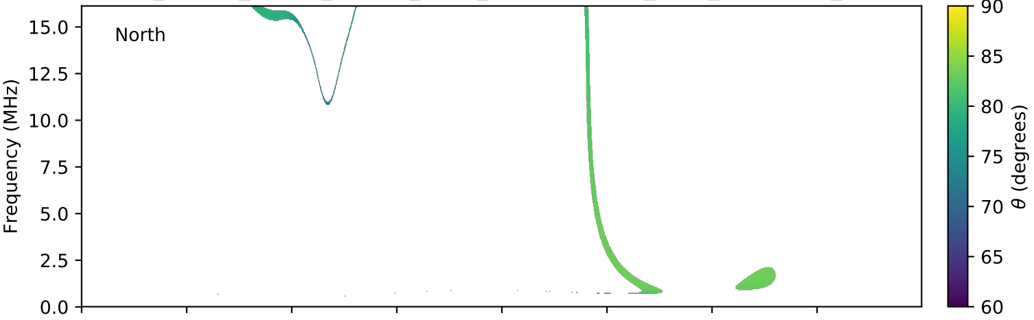
expres_cassini_jupiter_europa_isaac_lossc-wid1deg_3kev_20010409_v01.cdf
