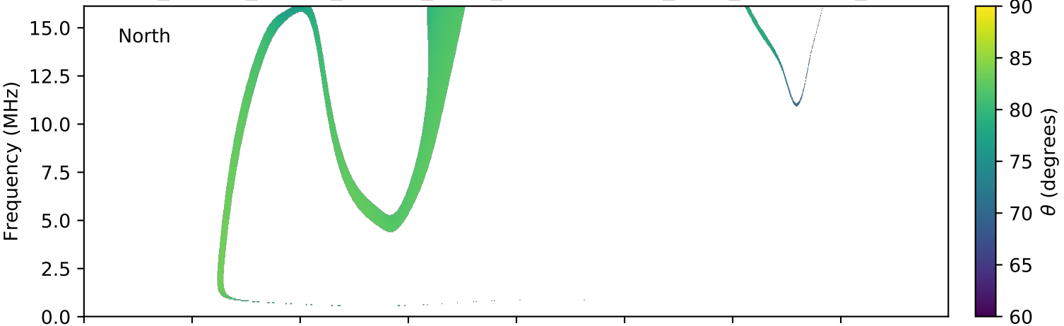
expres_cassini_jupiter_europa_isaac_lossc-wid1deg_3kev_20010408_v01.cdf
