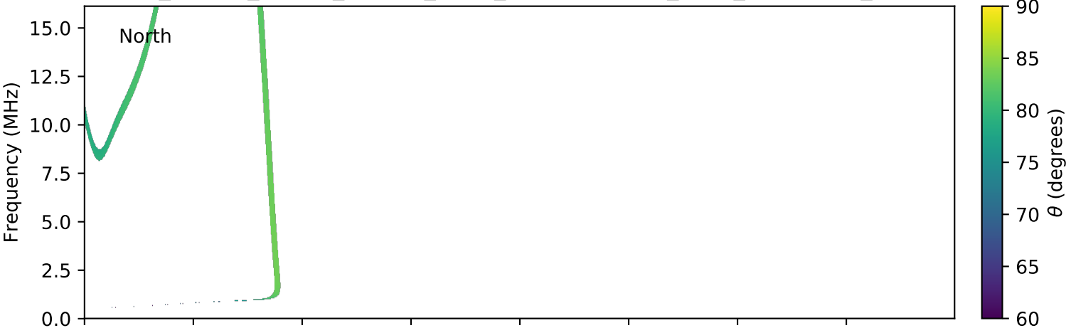
expres_cassini_jupiter_europa_isaac_lossc-wid1deg_3kev_20010406_v01.cdf
