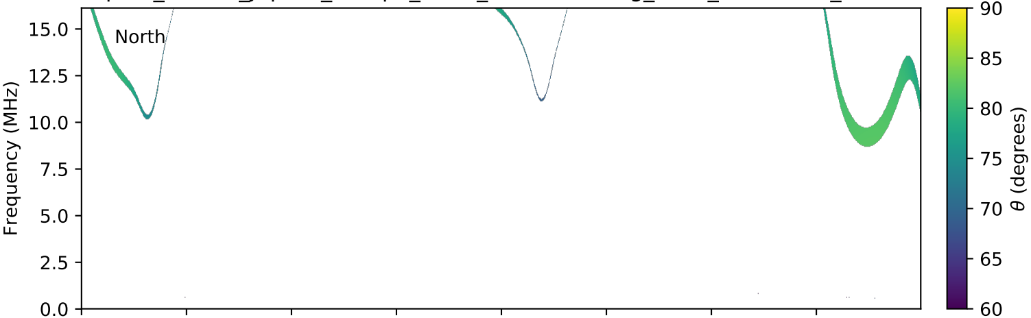
expres_cassini_jupiter_europa_isaac_lossc-wid1deg_3kev_20010405_v01.cdf
