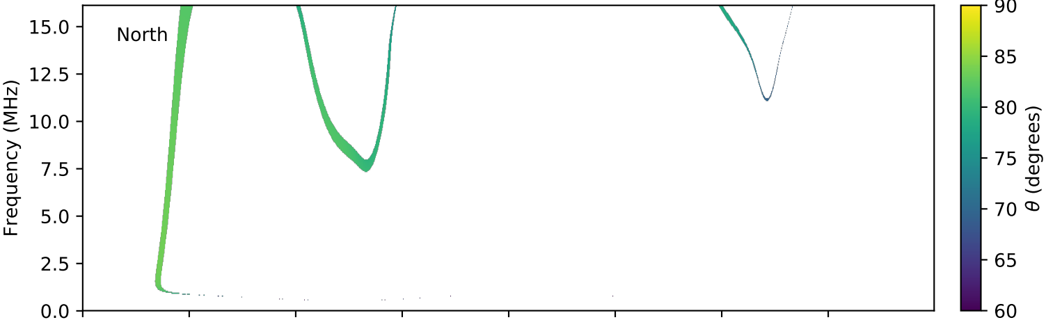
expres_cassini_jupiter_europa_isaac_lossc-wid1deg_3kev_20010401_v01.cdf
