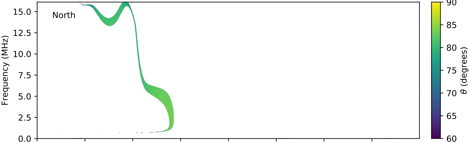
expres_cassini_jupiter_io_isaac_lossc-wid1deg_3kev_20010326_v01.cdf
