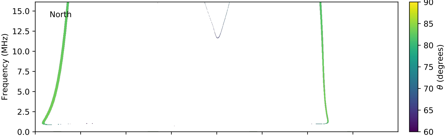
expres_cassini_jupiter_io_isaac_lossc-wid1deg_3kev_20010322_v01.cdf
