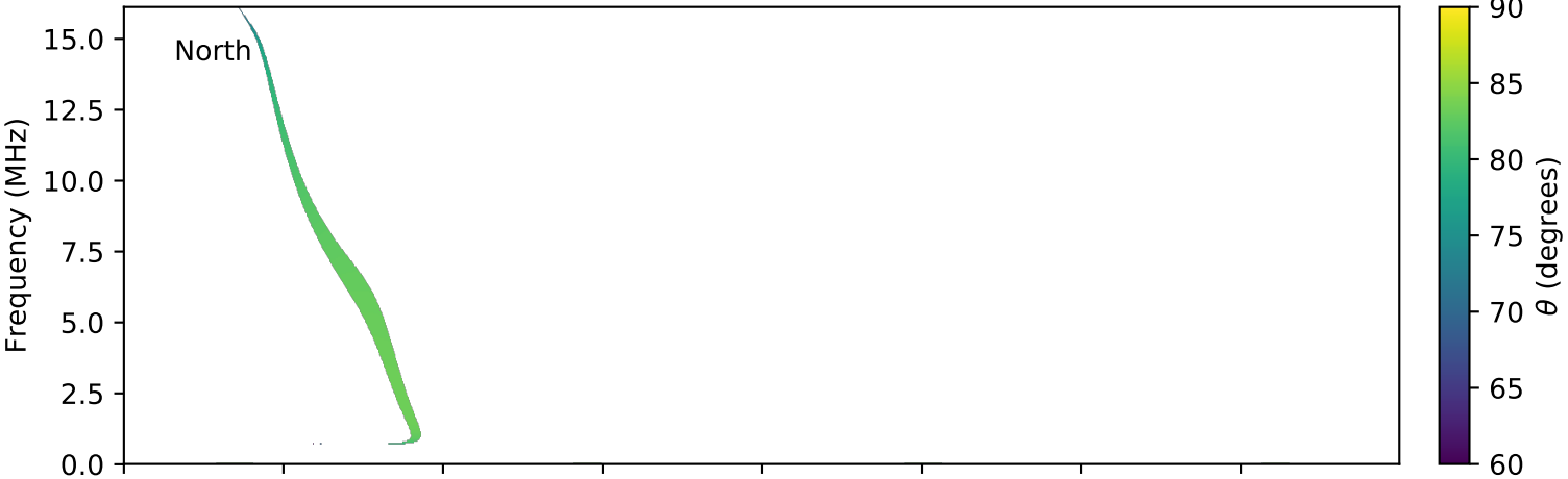
expres_cassini_jupiter_io_isaac_lossc-wid1deg_3kev_20010319_v01.cdf
